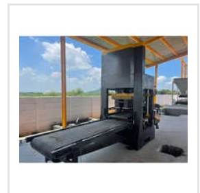
Mild Steel Fly Ash Brick Making Machine
